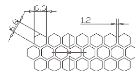
Hexagonal hole pattern perforation with 71%
