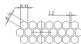
Hexagonal hole pattern perforation with 71%
