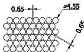
Round hole pattern perforation with 70%
